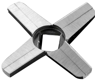
Bimetallic knife mod. "SALVADOR" with braze welded HSS inclined inserts mod. 22 - h 12,5 mm mod. 32 - h 13,4 mm mod. 42 (52) - h 18,7 mm
