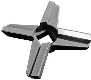
Bimetallic knife mod. "USA" with braze welded HSS inclined inserts mod. 32 - h 18,6 mm mod. 42 (52) - h 20 mm
